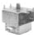
Power Rating: 700-850 Watts Peak Anode Voltage: 4.1 KV Antenna: Standard 30 mm #47-229 $34.50
