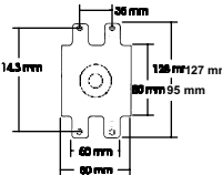
Power Rating: 700-850 Watts Peak Anode Voltage: 4.1 KV Antenna: Standard 30 mm #47-232 $37.90
