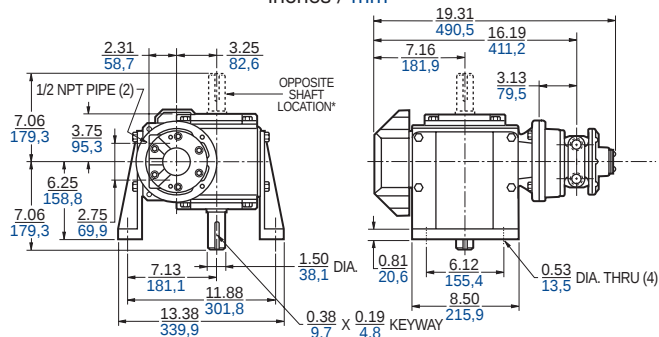
“C” Mounting 6AM-22A-GC40 (standard shaft) / *6AM-22A-GG40 (opposite shaft) inches / mm
