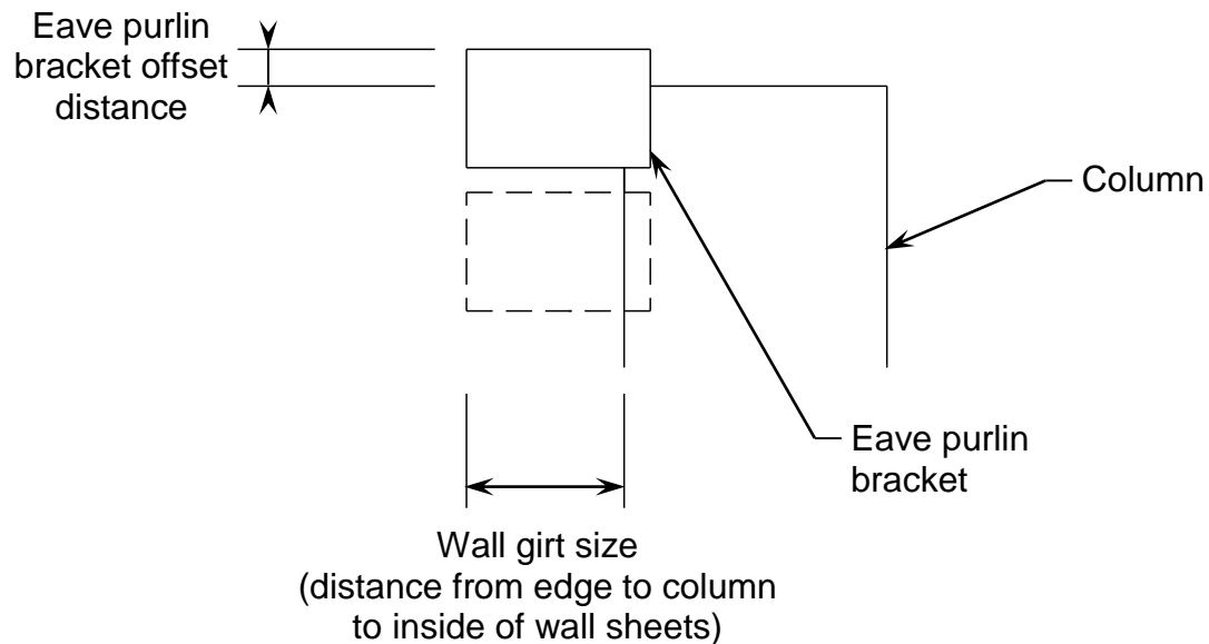
Eave Purlin Bracket Offset Table (continued on next page)
