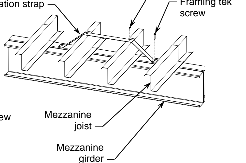
Mezzanine Joist Installation
