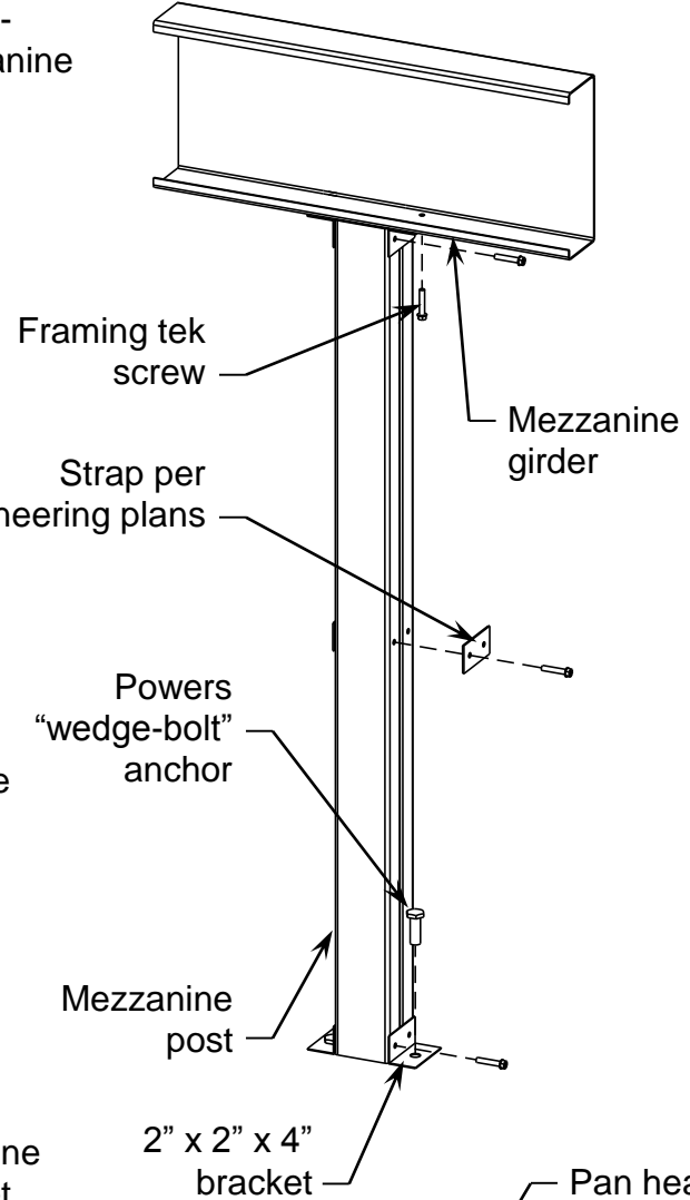
Front-To-Front Mezzanine Post Installation
