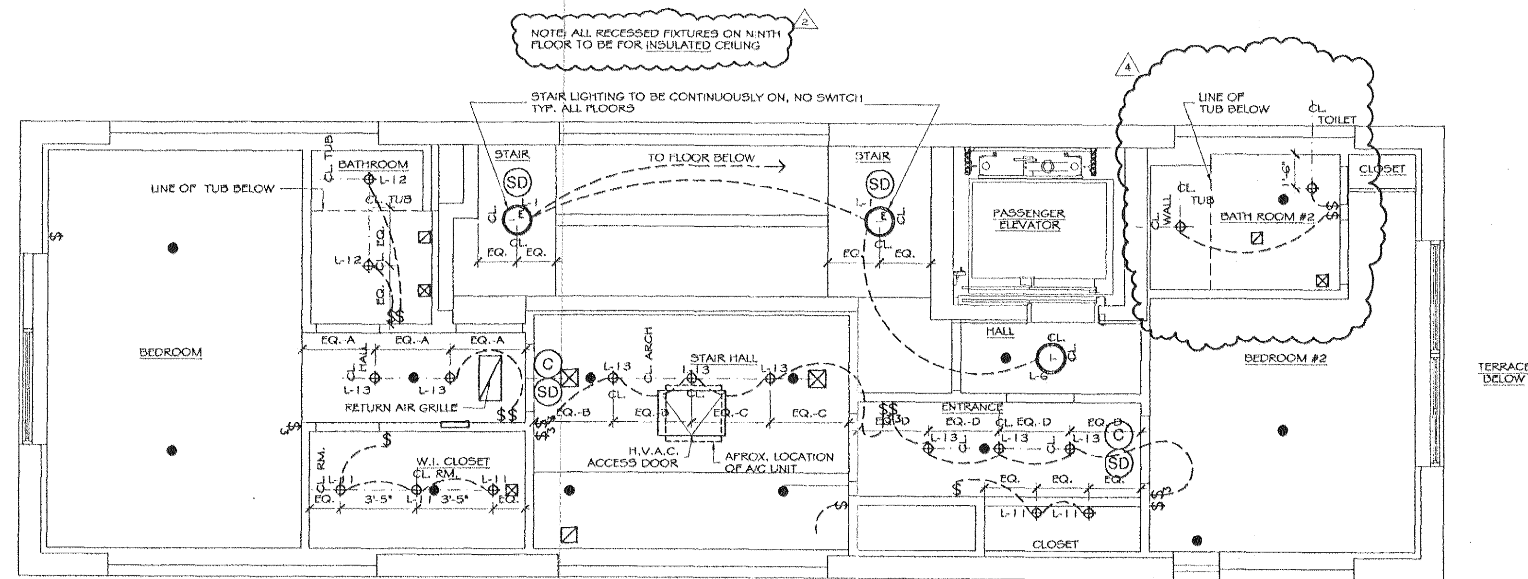
LIGHTING PLAN
