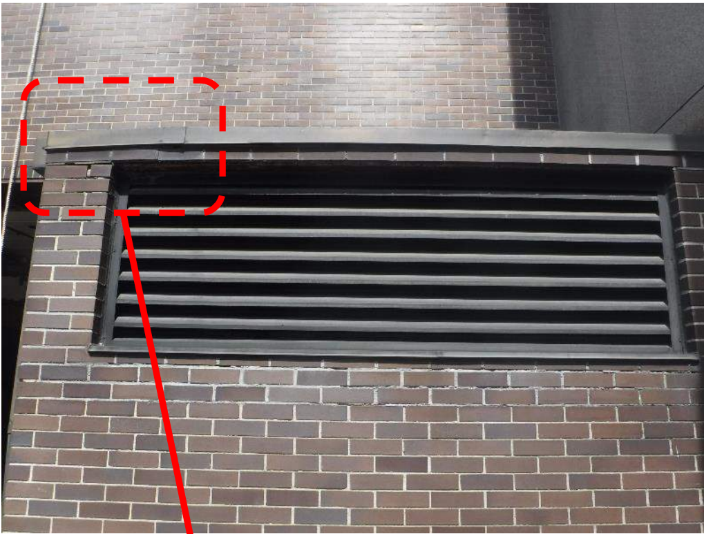
Detail Photo No. 19 - Overall view of South Elevation, masonry façade at Loading Dock entry.
