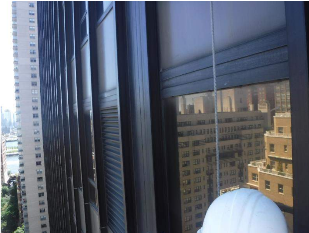
Detail Photo No. 8 – Overall view of North Elevation curtain wall detailing.
