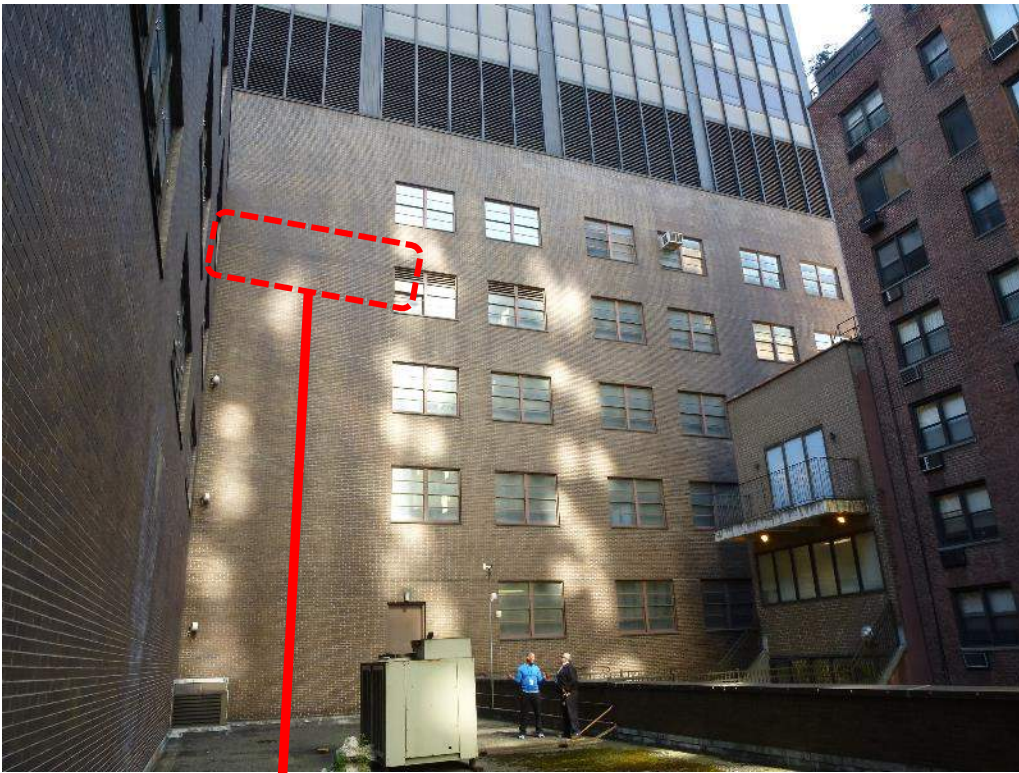
Detail Photo No. 27 - Overall view of West Elevation, lower floors, masonry facade.
