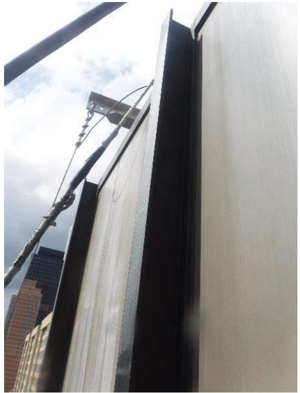
Detail Photo Nos. 17a & b - Overall view of South Elevation, exterior face of 8 th Floor Setback roof parapet at left; Main Roof parapet at right.
