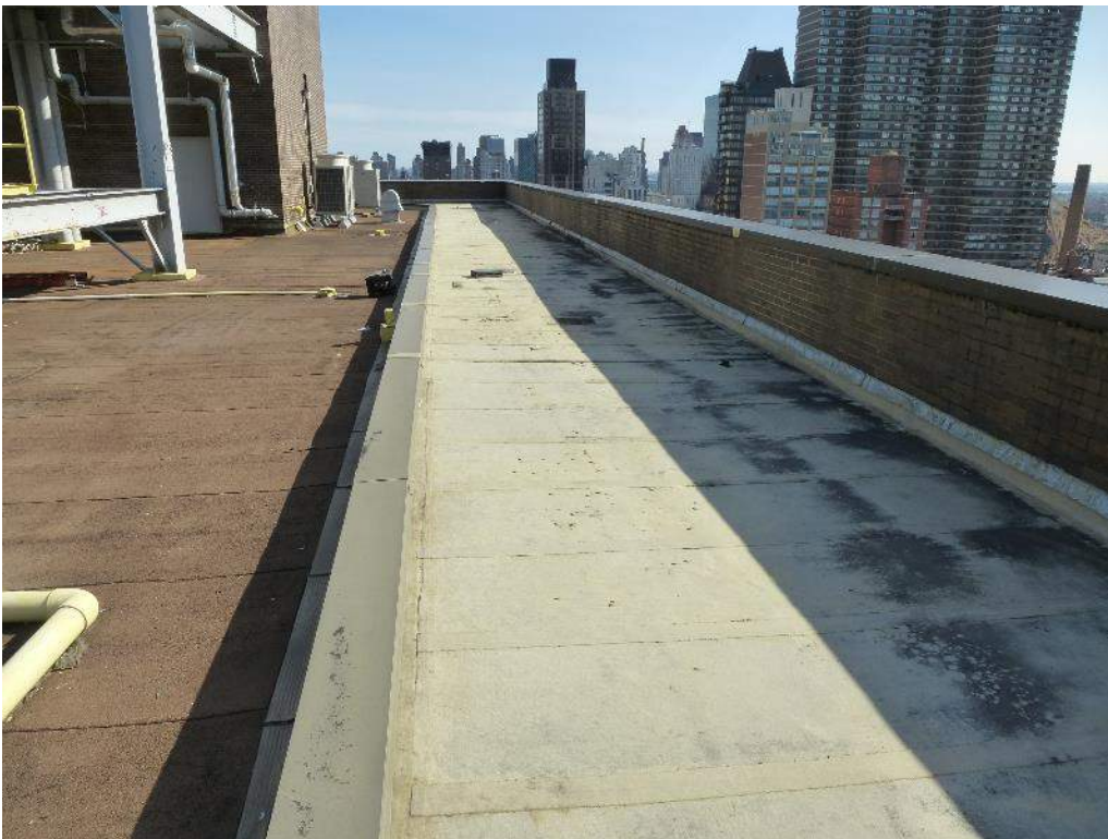
Detail Photo No. 34 – Main Roof looking south at window washing track.
