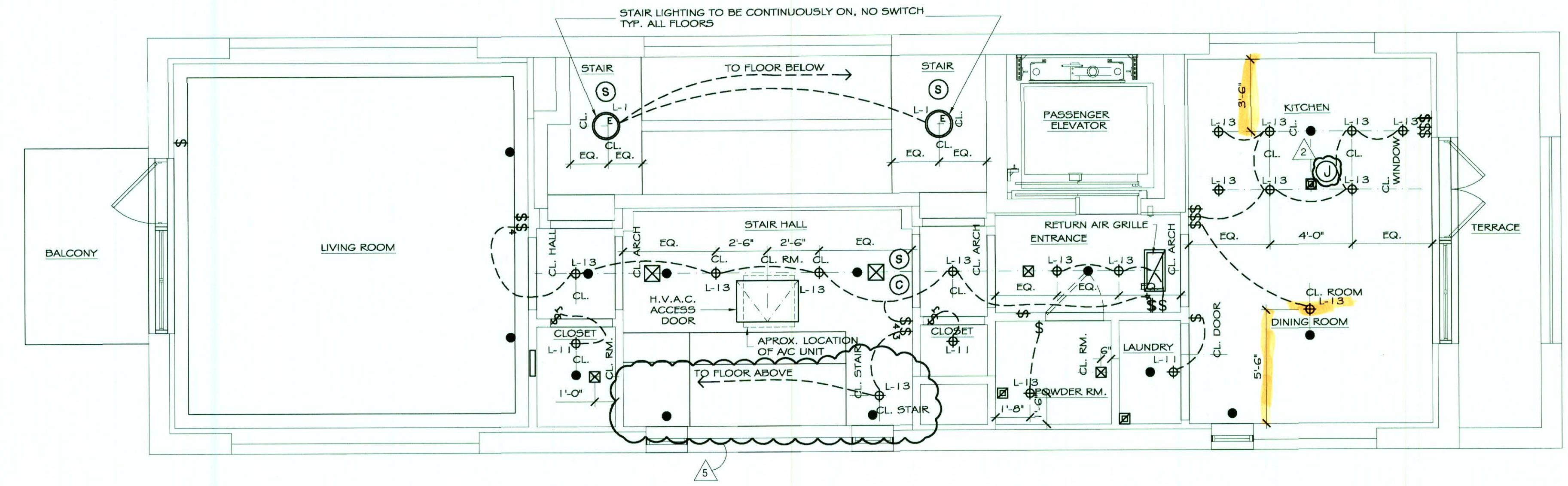
LIGHTING PLAN 1/4" = 1'-0"
