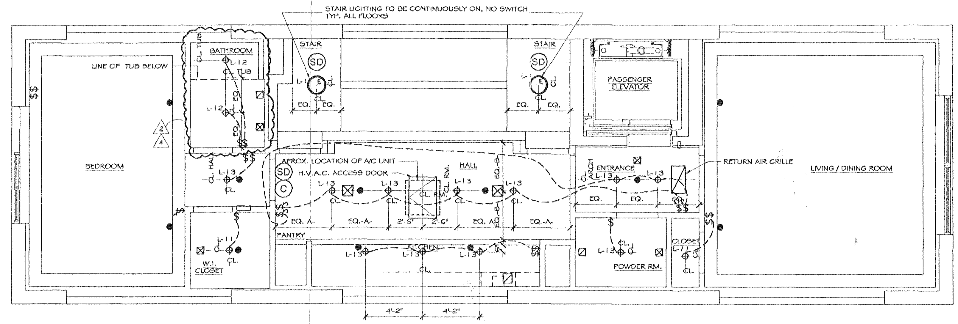
LIGHTING PLAN 1/4" = 1'-0"
