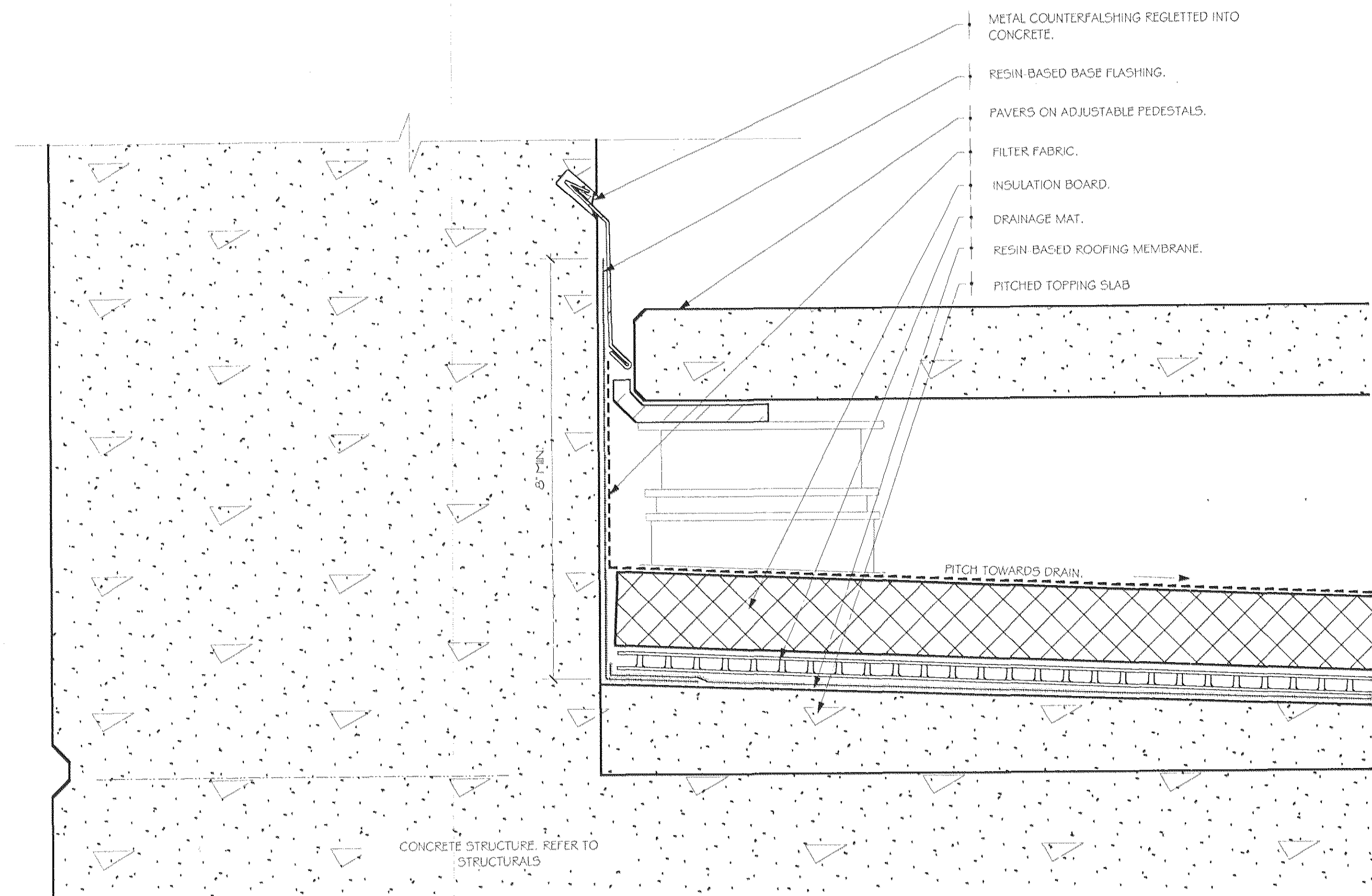
1 SECTION DETAIL AT CAST CONCRETE PARAPET WALL
