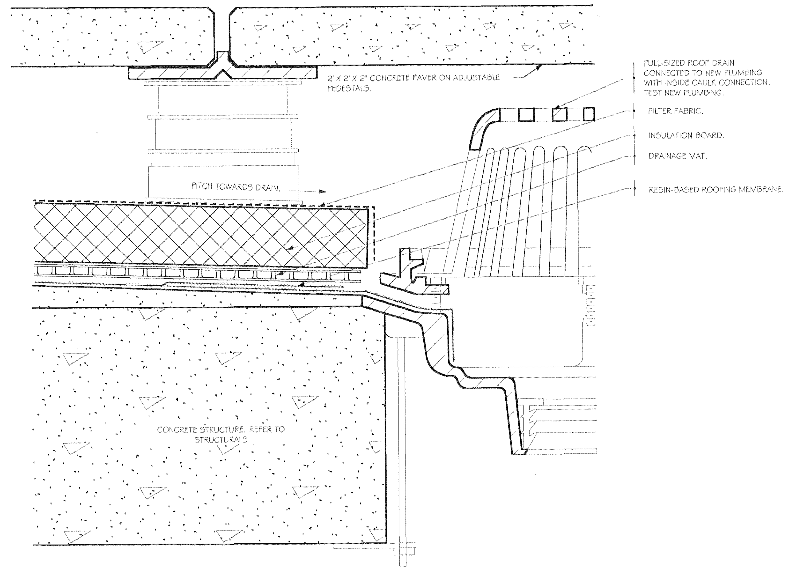
3 SECTION DETAIL AT ROOF AND TERRACE DRAIN
