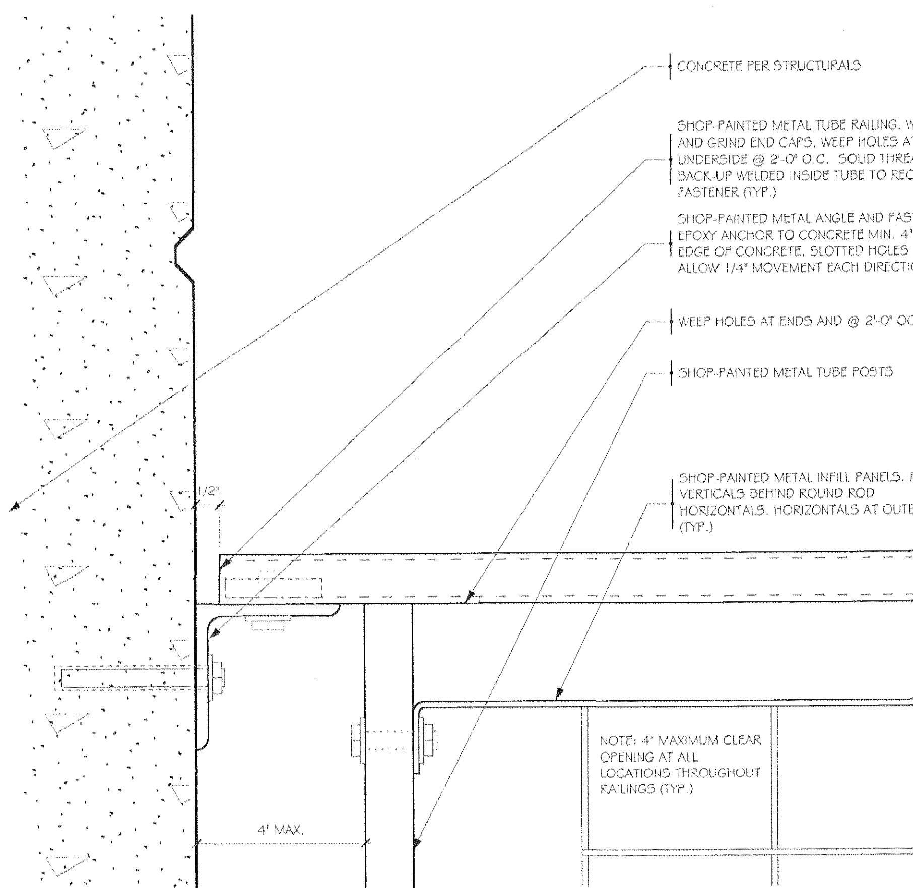
1 DETAIL - TYPICAL BALCONY RAILING @ WALL SCALE: HALF FULL SIZE
