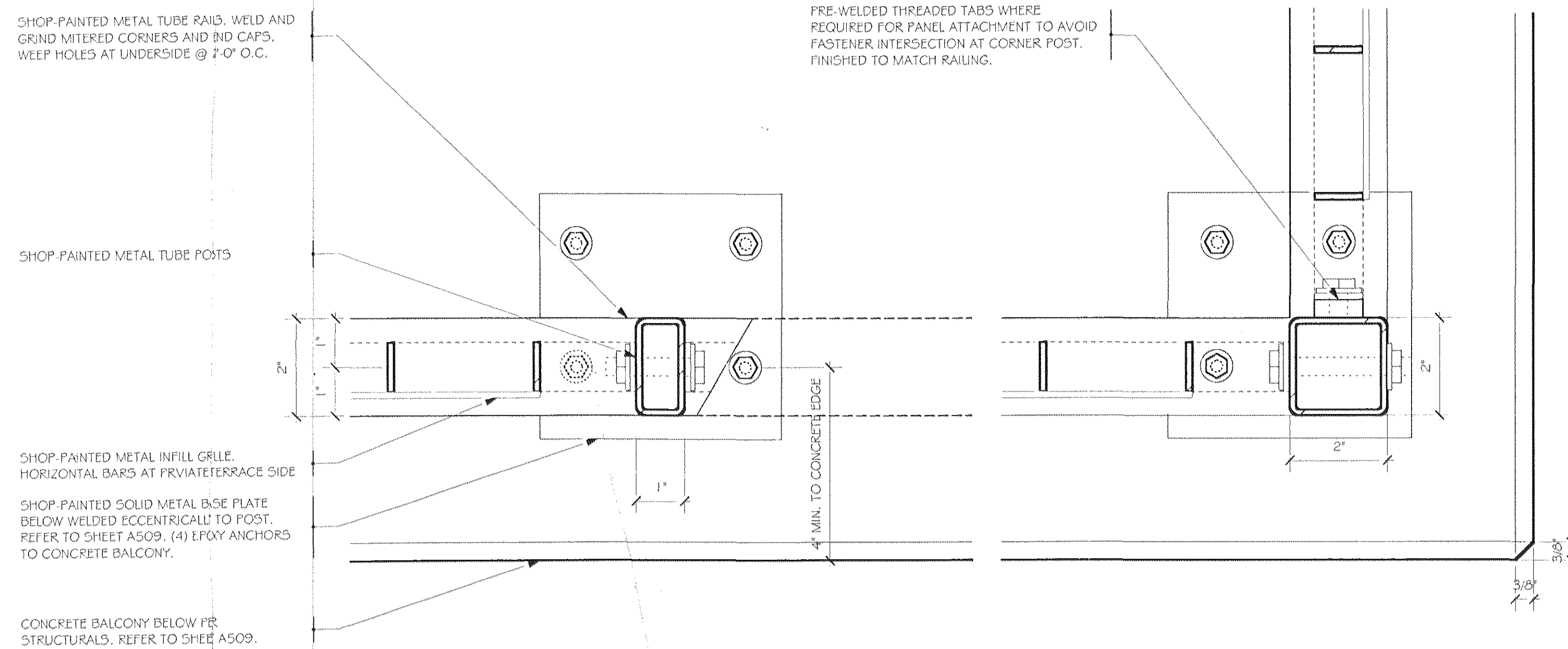
3 PLAN SECTION DETAIL - TYPICAL BALCONY RAILING SCALE: HALF FULL SIZE
