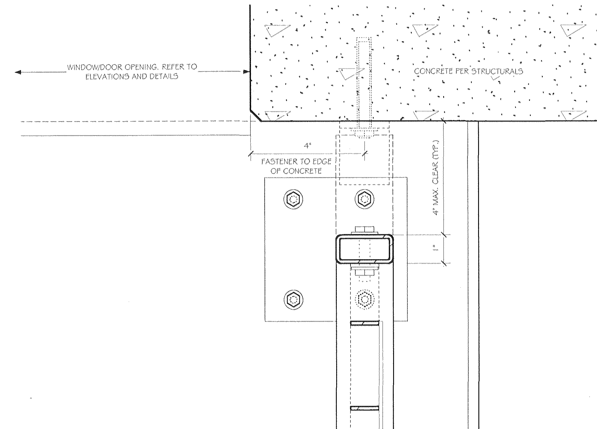
2 SECTION DETAIL - TYPICAL BALCONY RAILING SCALE: HALF FULL SIZE
