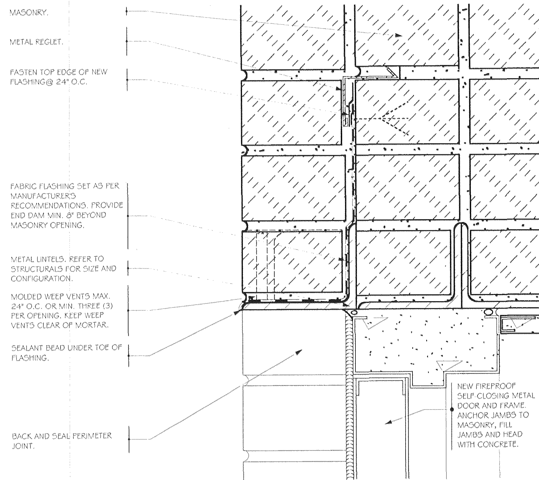
1 SECTION DETAIL - LOOSE LAID LINTEL
