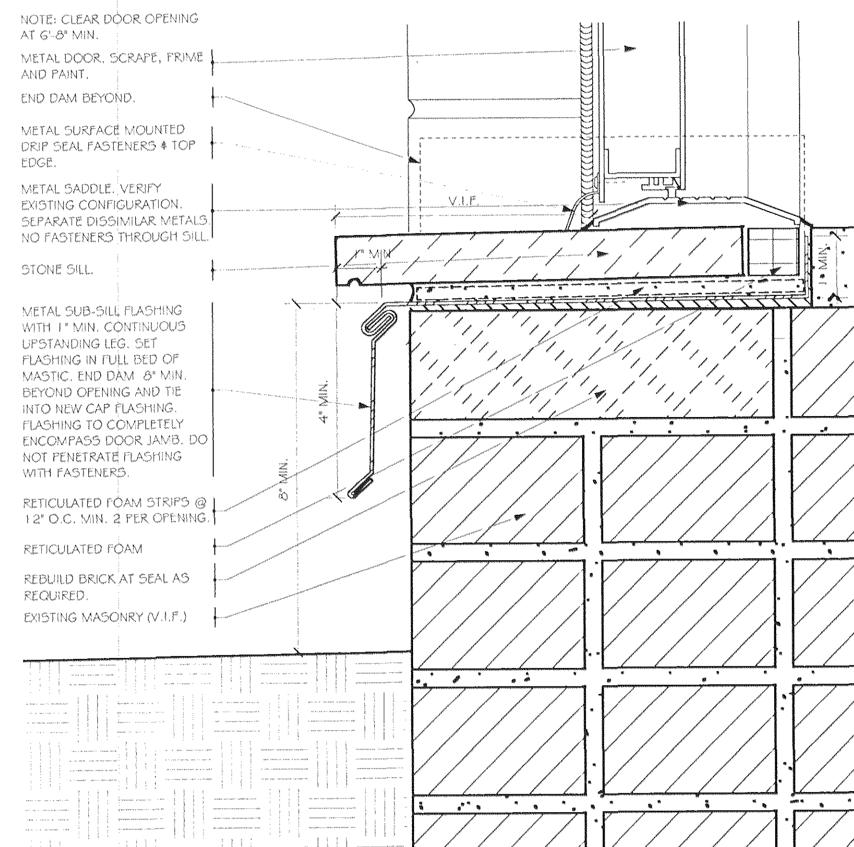
2 SECTION DETAIL - DOORSILL
