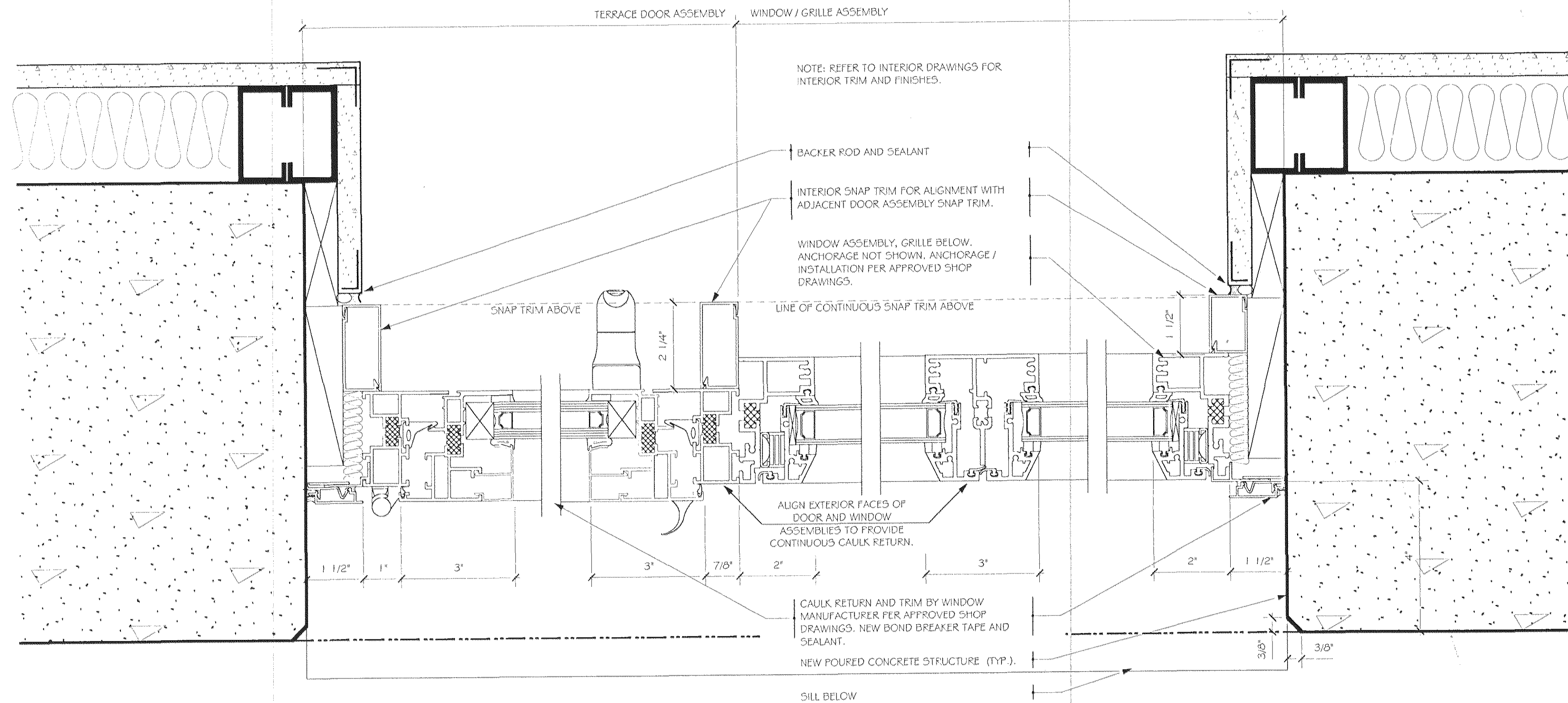
1 PLAN SECTION - TYPICAL BALCONY WINDOW/DOOR ASSEMBLY
