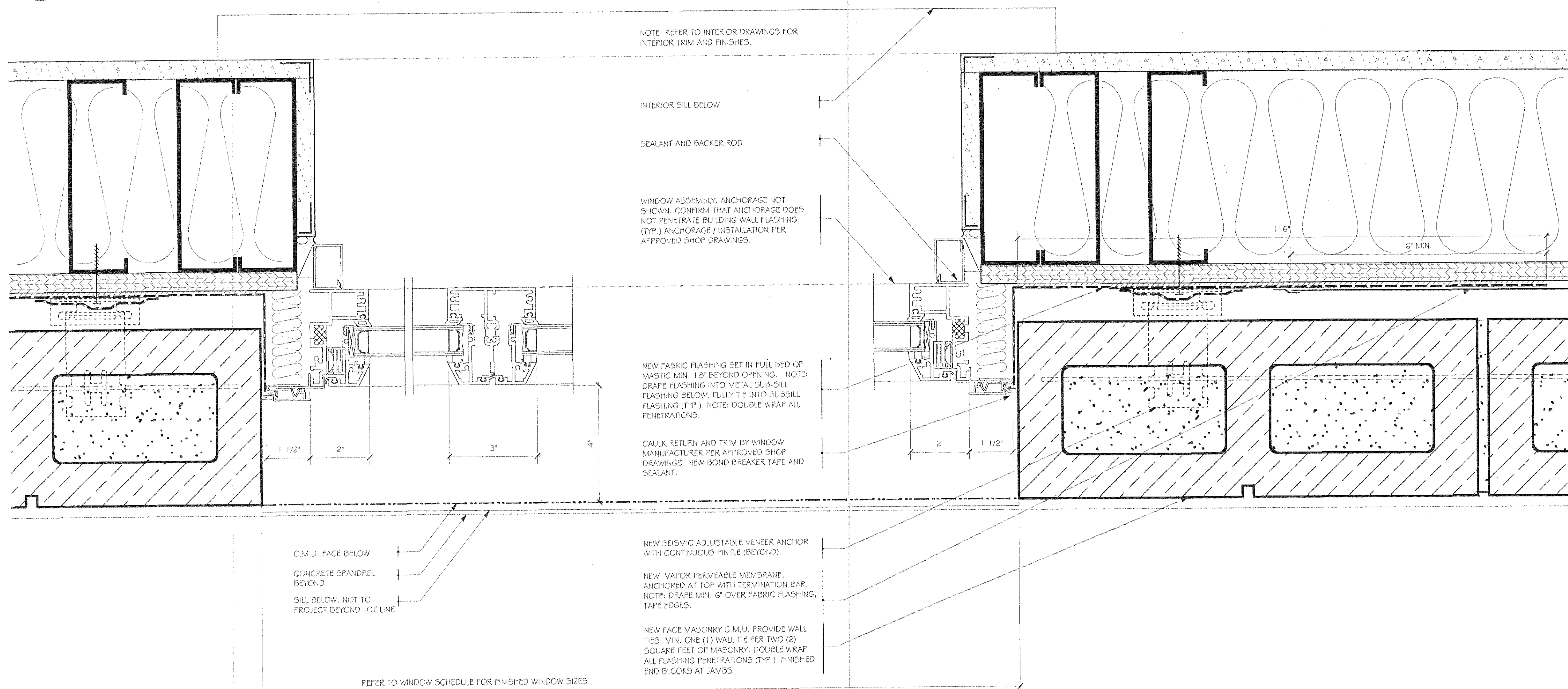
2 PLAN SECTION - WINDOW AT C.M.U. WALL
