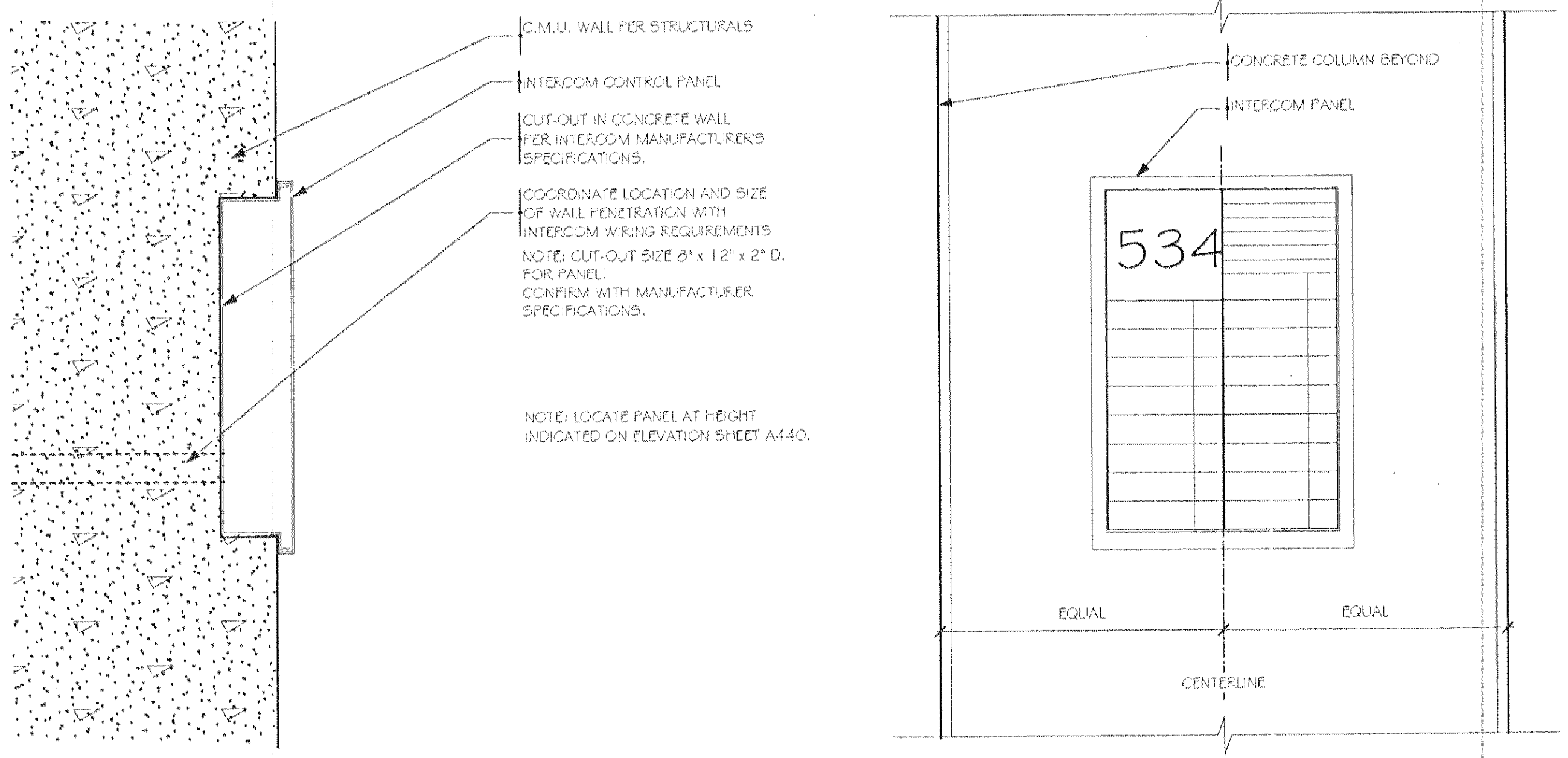
1 SECTION DETAIL - INTERCOM PANEL SCALE: 3" = 1'-0"
