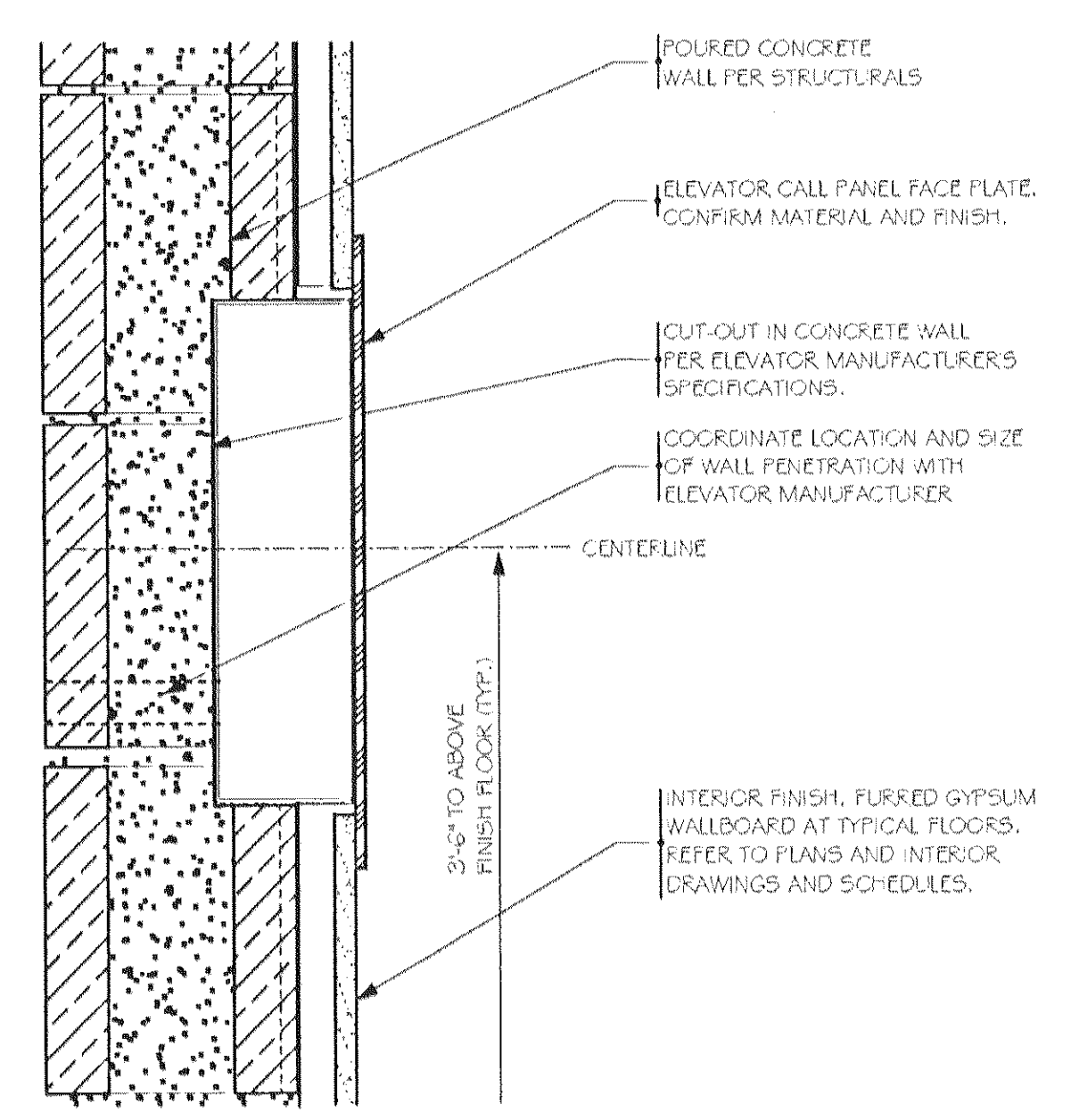
4 SECTION DETAIL - ELEVATOR CALL PANEL SCALE: 3" = 1'-0"
