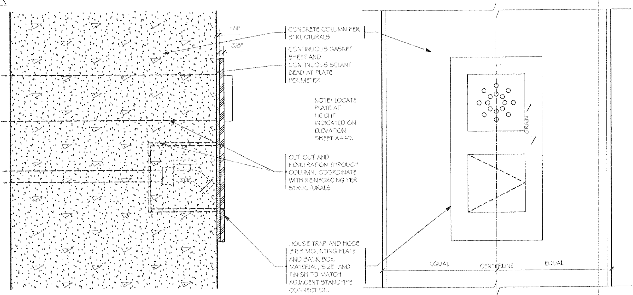
3 SECTION DETAIL - HOUSE TRAP FACE PLATE SCALE: 3" = 1'-0"
