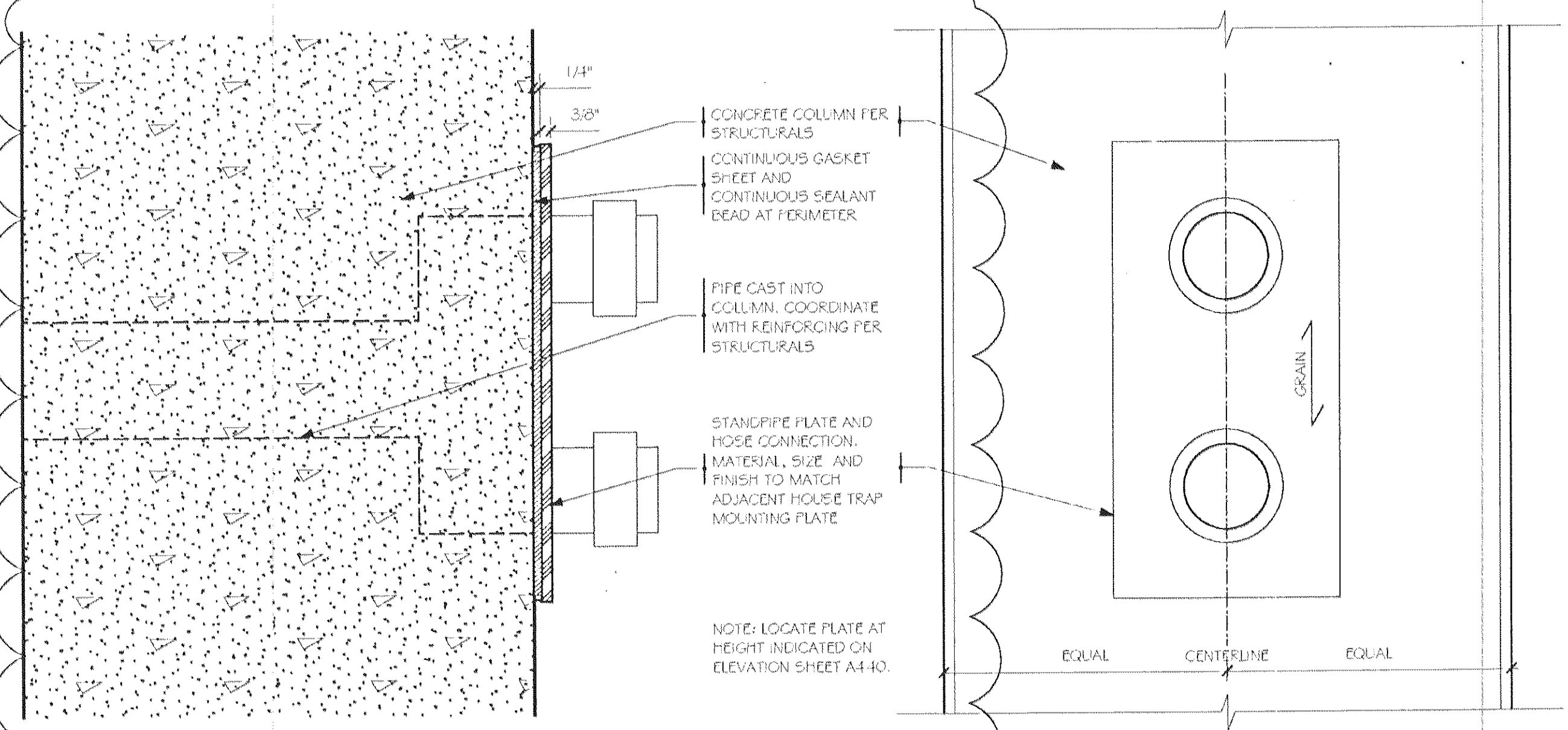
2 SECTION DETAIL - STANDPIPE CONNECTION SCALE: 3" = 1'-0"
