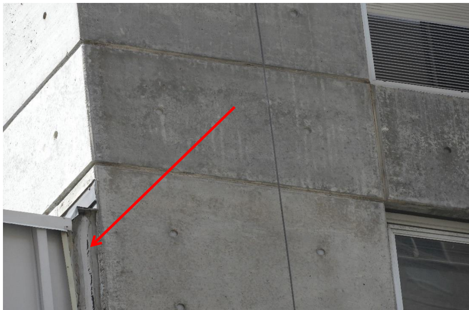
Photo 4. Split caulking at building joint line.
