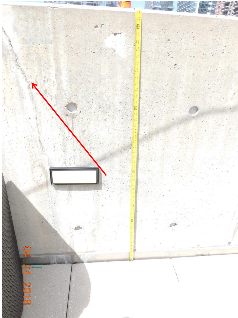
Photo 5. Vertical crack at interior of parapet.
